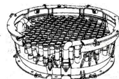
Moderatortanklock
