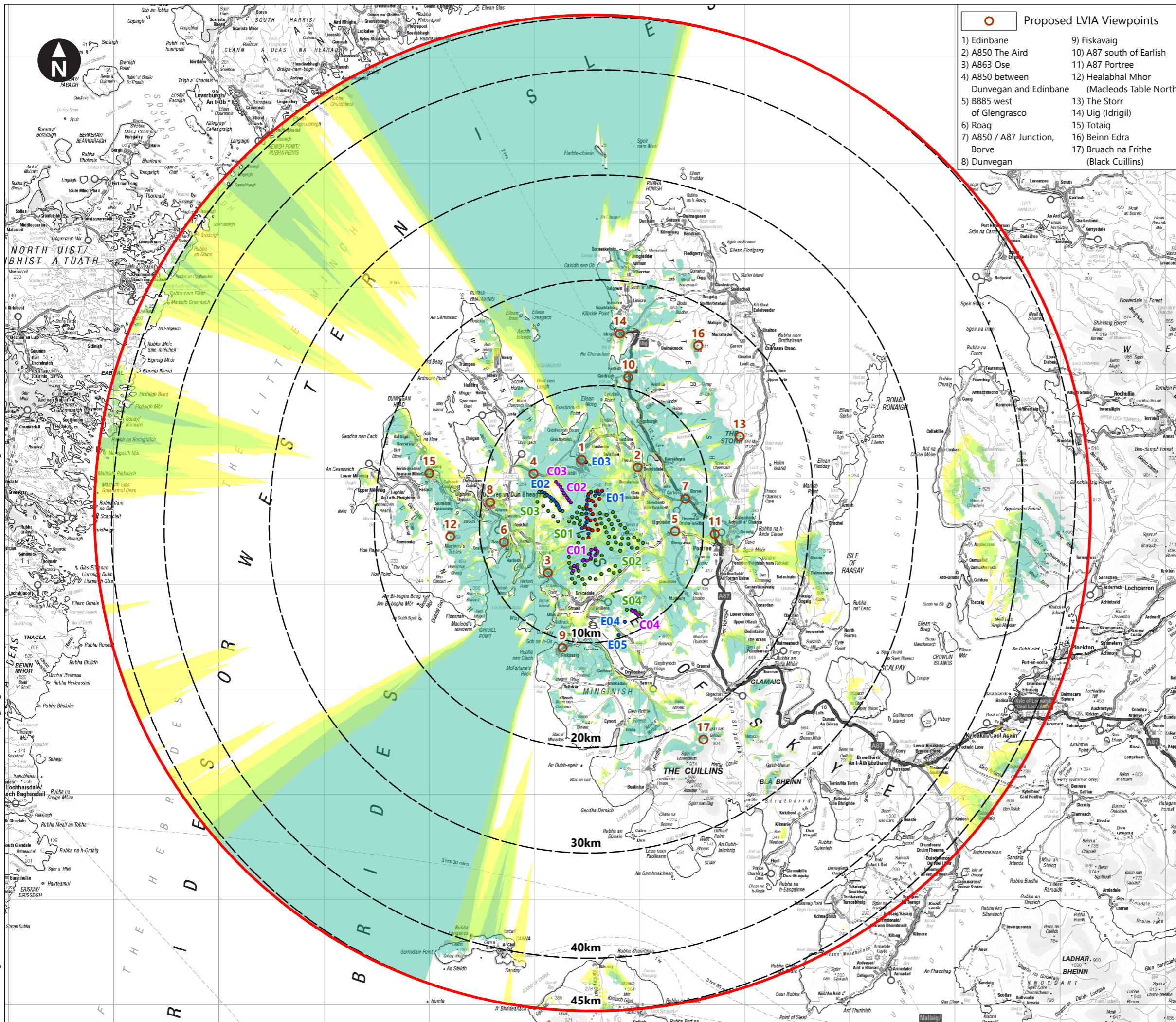
Figure 6.1 LVIA Study Area and ZTV of Proposed Development (to Blade Tip) with Viewpoint Locations and Cumulative Wind Farms within 45km
